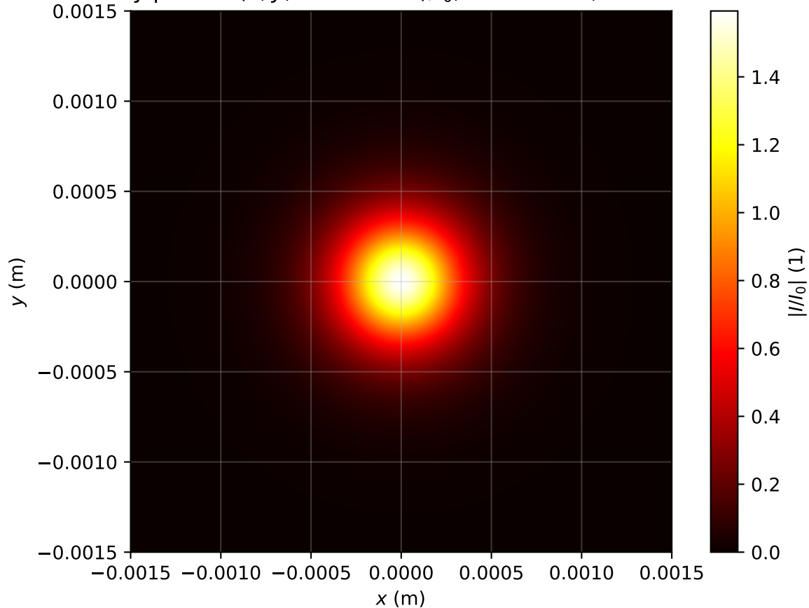
Intensity profile I(x, y, z = 2.786m)/I_0 , Pin=0.9Pcr, artificial time
